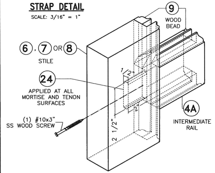
TYPICAL SASH INTERMEDIATE CONNECTION (EXTERIOR VIEW) SCALE: 3/16" = 1"
