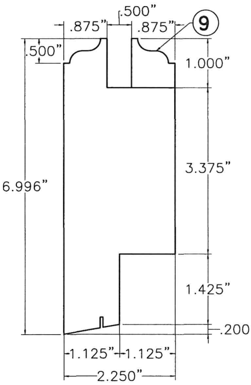
⑤ BOTTOM RAIL
