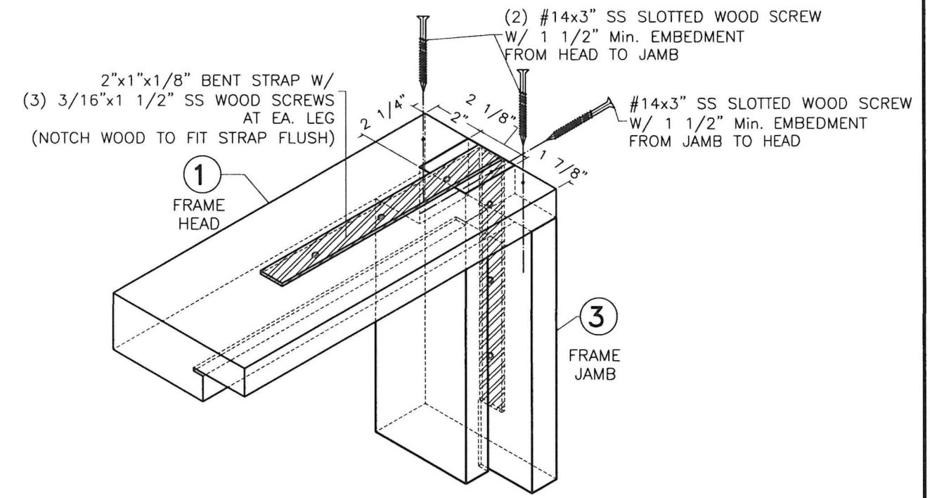
TYPICAL REGULAR FRAME TOP CONNECTION SCALE: 3/16" = 1"
