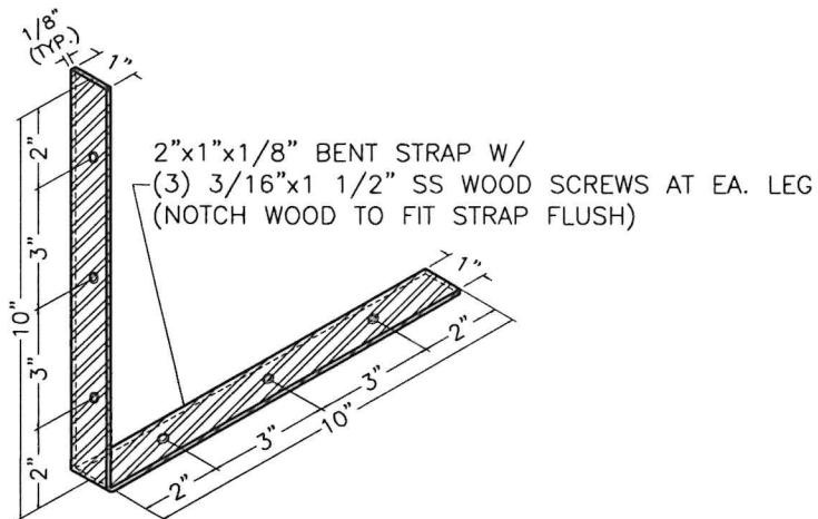
STRAP DETAIL SCALE: 3/16" = 1"
