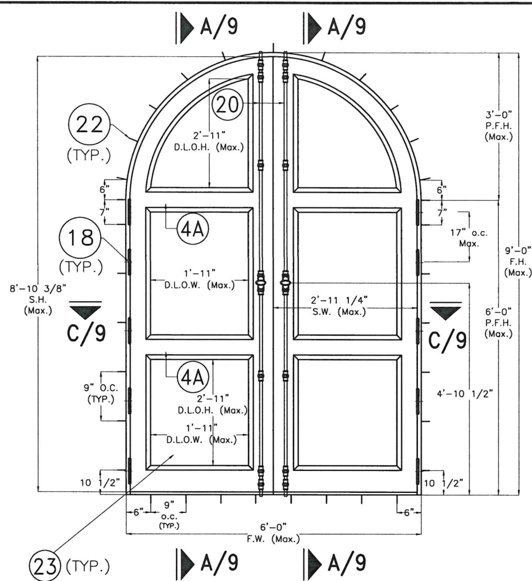
FULL ARCHED OUTSWING DOOR (XX)
