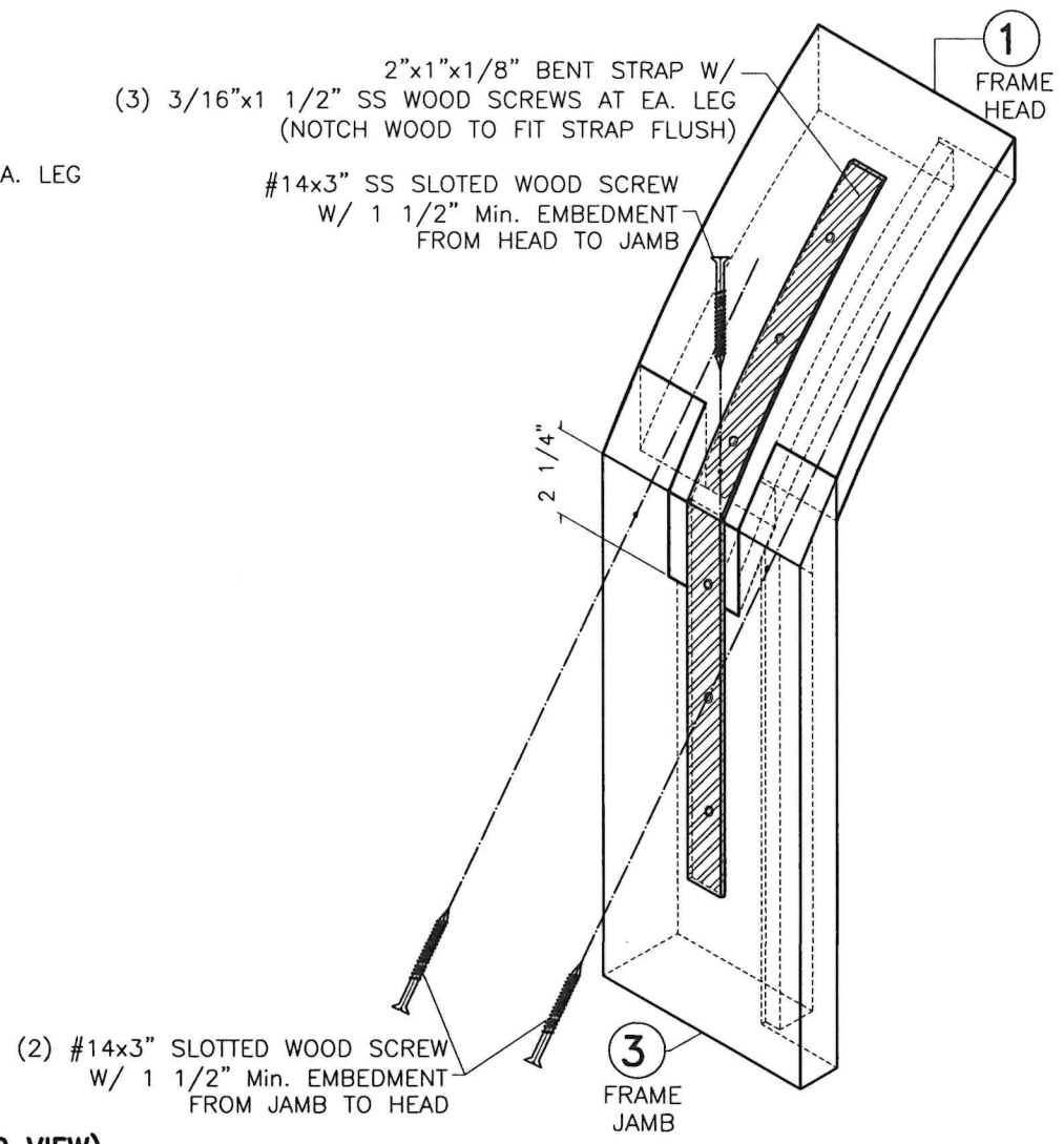
TYPICAL ARCHED/ELLIPTICAL FRAME TOP CONNECTION SCALE: 3/16" = 1"
