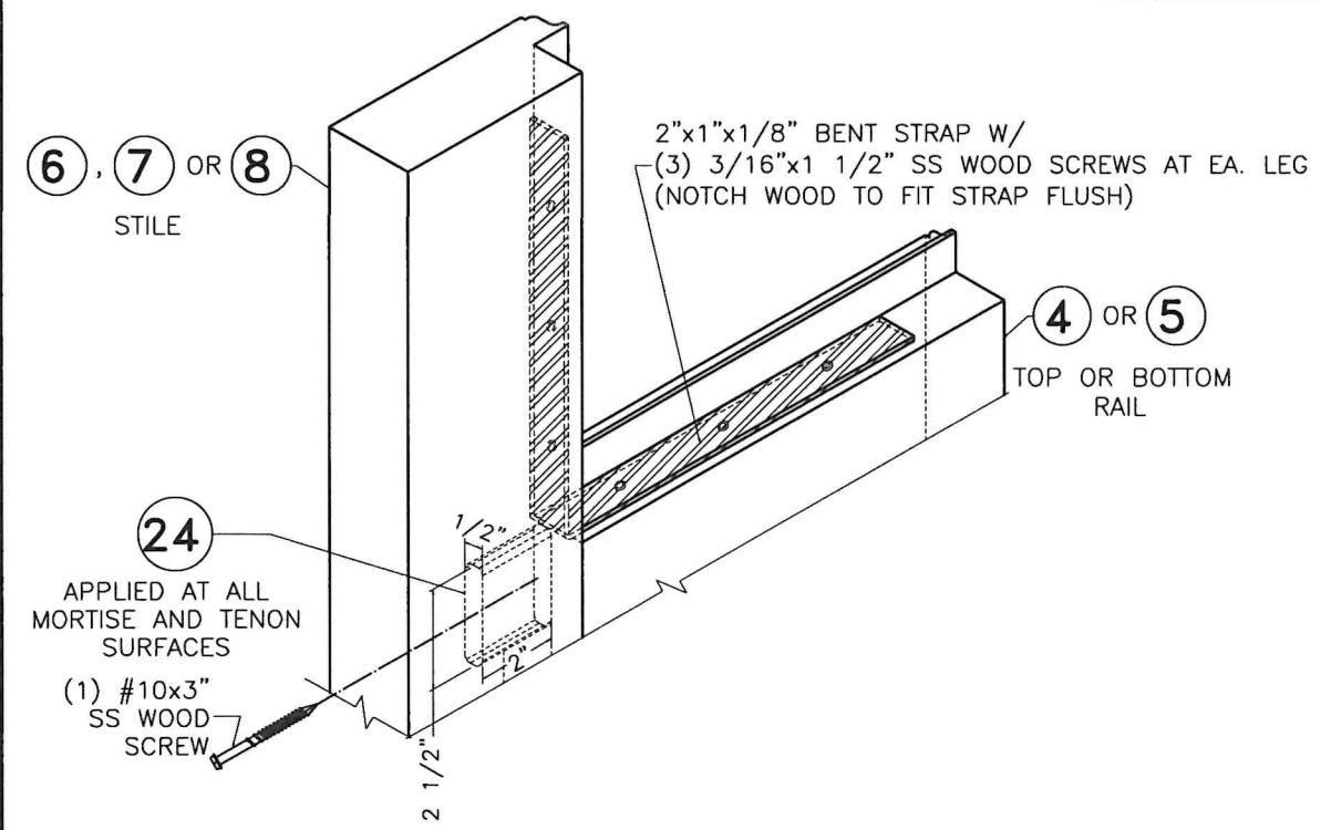
TYPICAL SASH TOP/BOTTOM CONNECTION (EXTERIOR VIEW) SCALE: 3/16" = 1"
