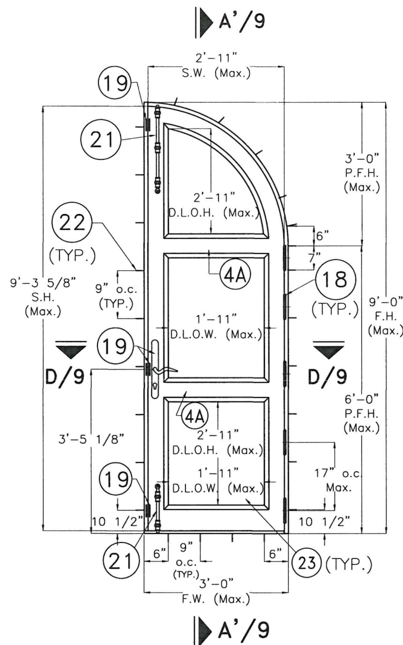
SINGLE 1/2 ARCHED OUTSWING DOOR (X)
