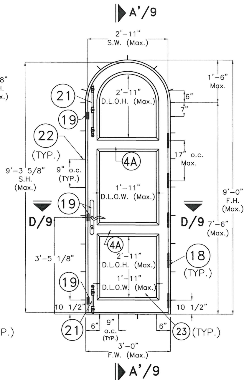
SINGLE FULL ARCHED OUTSWING DOOR (X)
