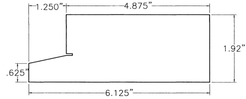
② FRAME SILL
