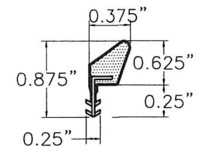
⑭ Q-LON WEATHER SEAL
