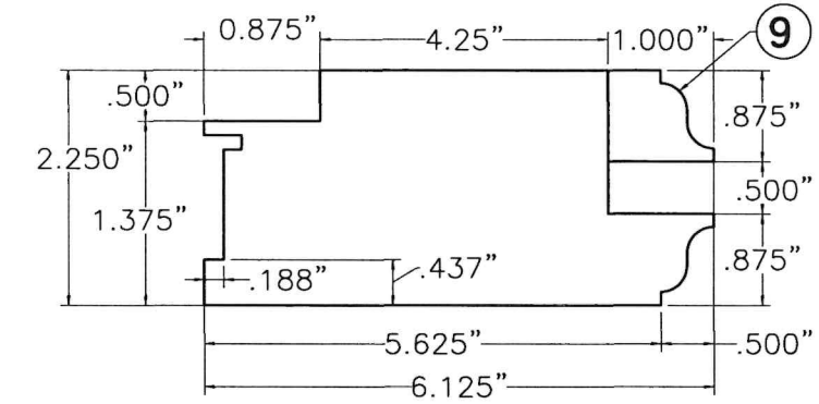
④ TOP RAIL, ⑥ HINGE STILE
