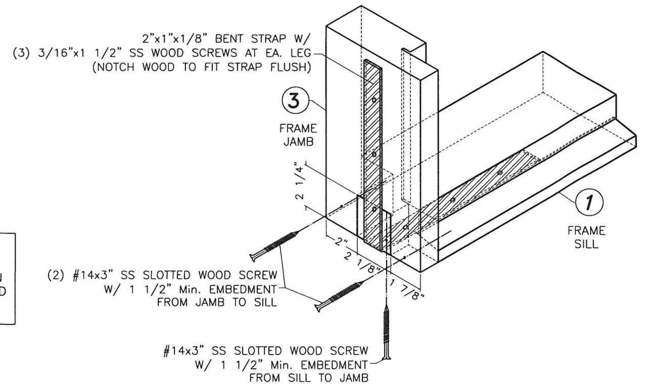
TYPICAL FRAME BOTTOM CONNECTION SCALE: 3/16" = 1"
