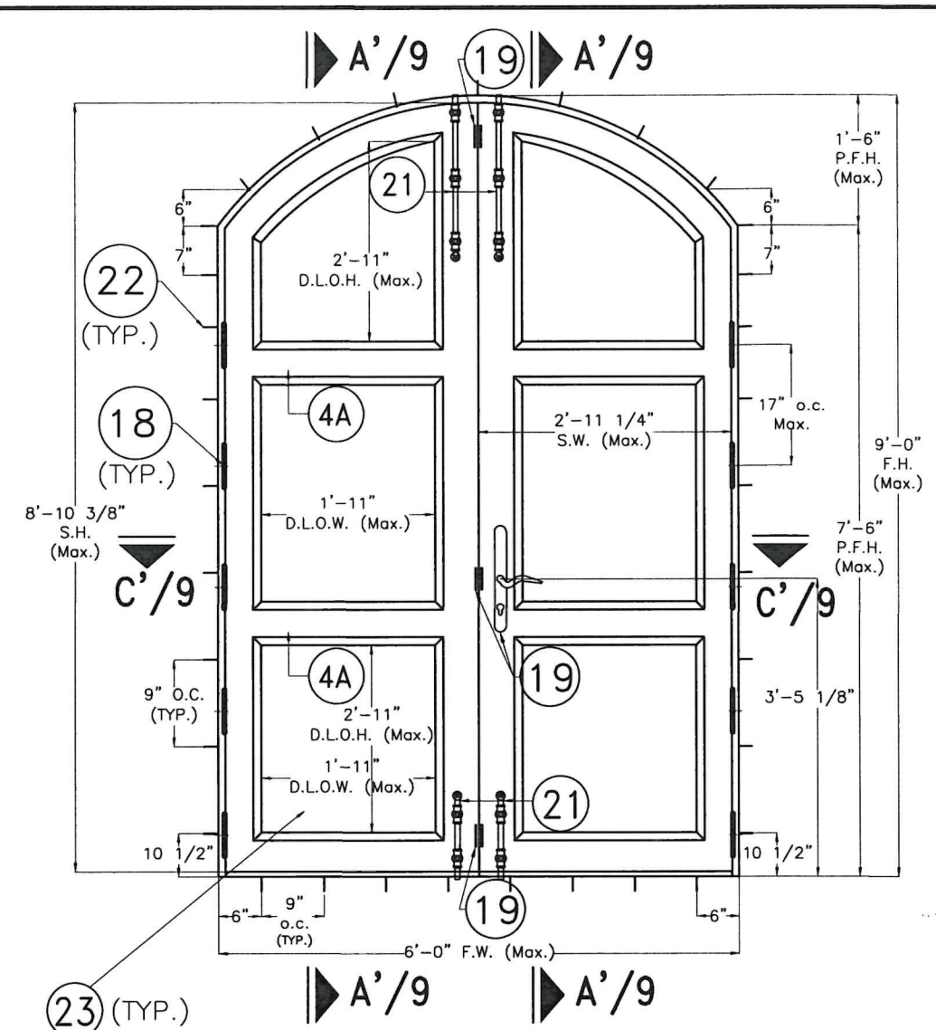
ELLIPTICAL OUTSWING DOOR (XX)
